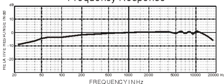
Frequency Response
