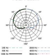
Polar Pattern
