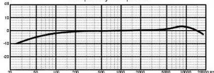
Frequency Response
