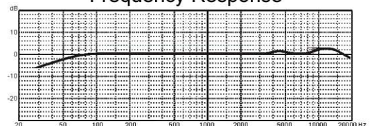
Frequency Response
