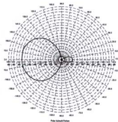
E-Plane Pattern
